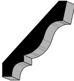
ABC 609 O/M CROWN 1 1/16" X 4 5/8"
